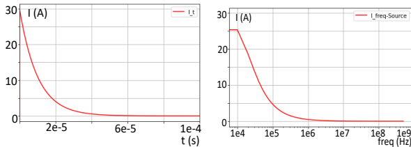
Figure 18. Bi-exponential signal 2 source in time and frequency domain
