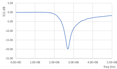
Figure 5. S_{11} parameter for the 25cm monopole Measurement
