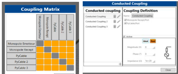
Figure 10. Radiated and conducted coupling definition
