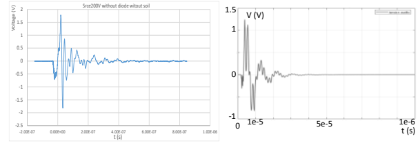
Figure 27. Reference: Measurement (left) and TEMSI-FD (right) simulation of the system without lossy soil
