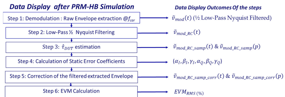
Figure 3. Principle of the design flow graph of the demodulation and EVM calculation after PRM-HB simulation.
