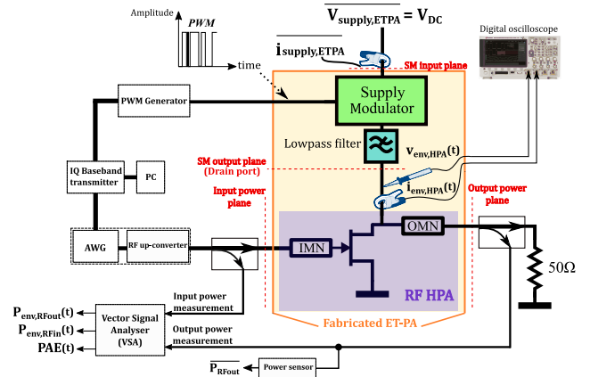
Fig. 1. ET-PA block diagram and its associated measurement setups.
