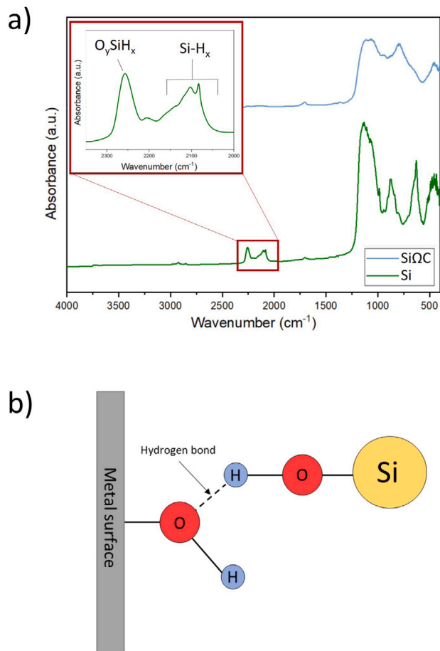
Fig. 9. (a) FTIR spectra of Si and SiO 2 C powders, (b) Schematic representation of hydrogen bond between Si particle and metal surface possibly causing the ejection issue.
