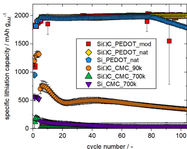
Fig. 5. Specific discharge capacity versus cycle number at 0.05C (4 initial cycles), and 0.2C (100 cycles) for tape-casted anodes. The measurements were performed at 30 °C. SiO x PEDOT mod - SiO x anode with PEDOT:PSS at modified pH of 10; SiO x PEDOT nat - SiO x anode with PEDOT:PSS at natural pH of 1.7; Si 2 PEDOT nat - Si anode with PEDOT:PSS at natural pH of 1.7; SiO x CMC 90k - SiO x anode with CMC of M_w \sim 90000 ; SiO x CMC 700k - SiO x anode with CMC of M_w \sim 700000 ; Si 2 CMC 700k - Si anode with CMC of M_w \sim 700000 .
