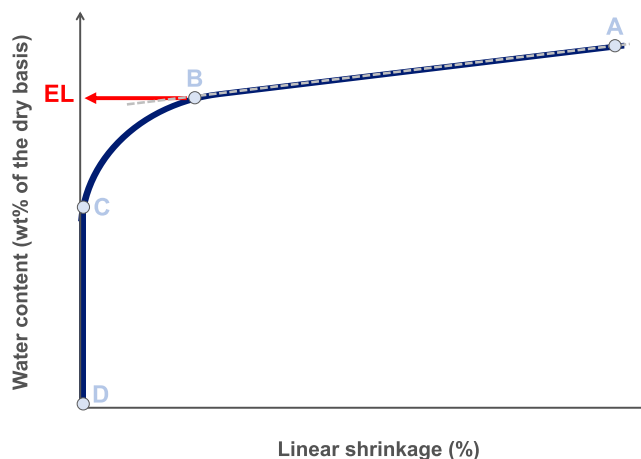
Fig. 1. Schematic representation of a typical Bigot curve.
