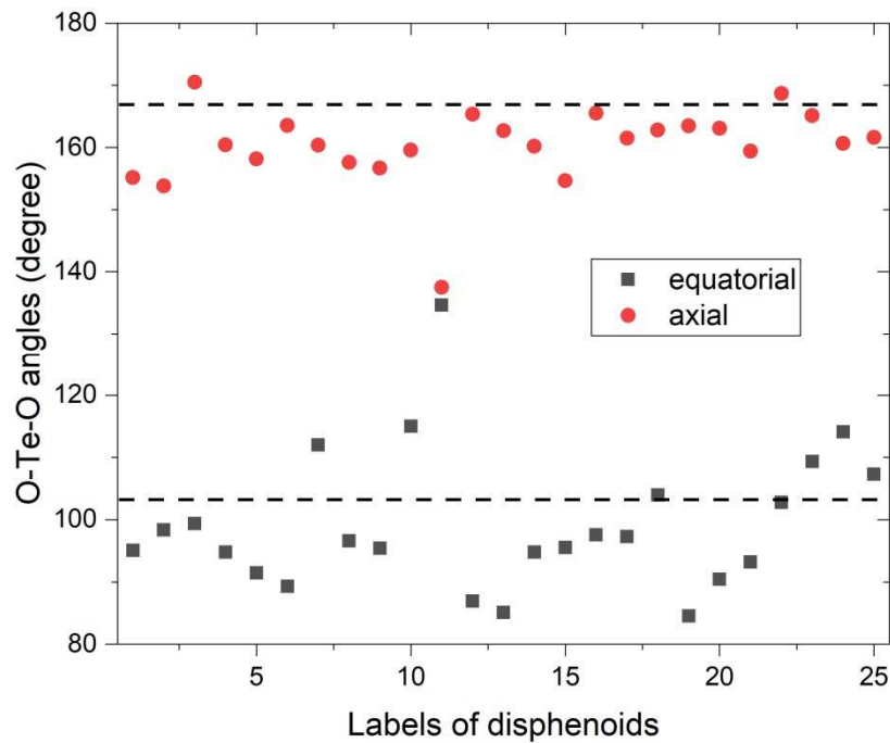
Fig 5. Valence angles between equatorial and axial Te-O bonds in the optimized structure of cluster III. Horizontal dashed lines indicate the angle values for the experimental paratellurite lattice.
