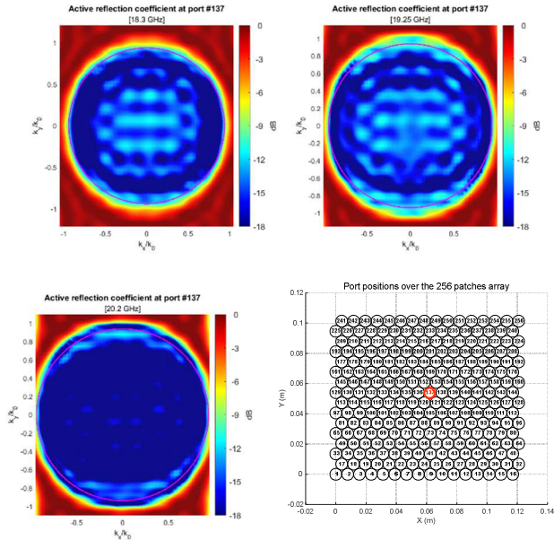
Fig. 3. Active reflection coefficients of the central cell (nr137) of the finite array for 18.3 GHz, 19.25 GHz and 20.2 GHz. The magenta circle represents the direction \theta_0=70^\circ . One can notice some ripples due to finite size but no reflection higher than -10 dB appears.
