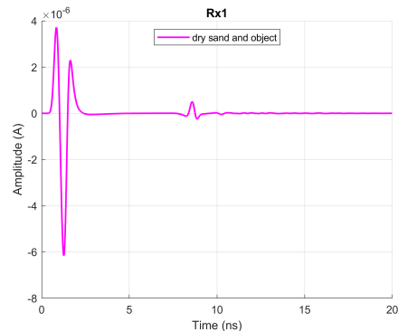
Fig 2: Example of the waveform of an A-scan captured by the receiving antenna. R_{x1}
