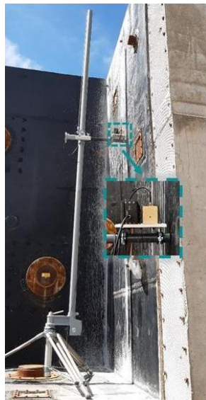
Figure 9: Measurement of the magnetic fields behind wall W1.
