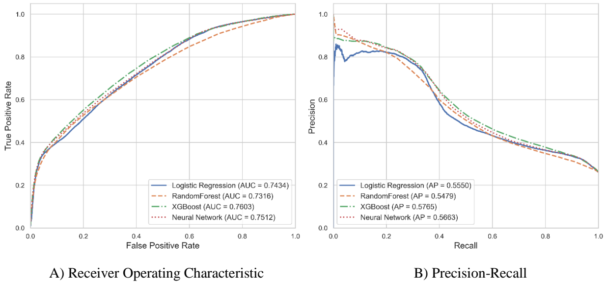
Figure A3.1: Receiver Operating Characteristic and Precision-Recall Curves
