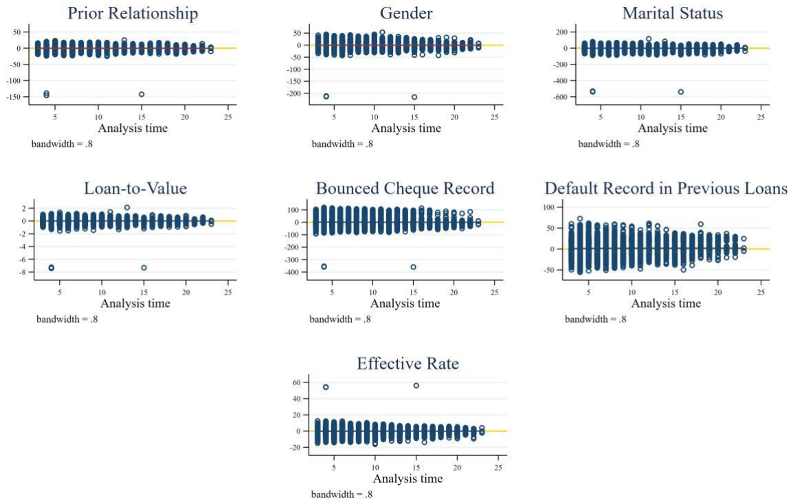
Figure A2.4: Test of Proportional Hazards Assumptions – Graphical Scaled Schoenfeld Residual
